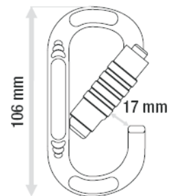
Automatic lock requires three actions: slide, twist and open.
