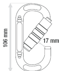
Automatic lock requires two actions: twist and open.
